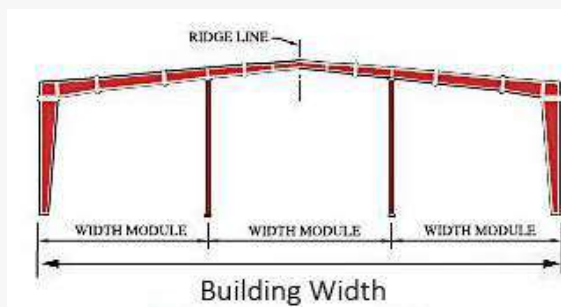
MULTI-SPAN '2'
