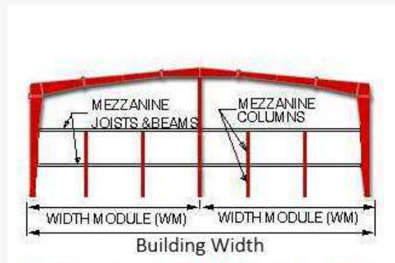
MULTI-SPAN WITH MEZZANINE FLOOR
