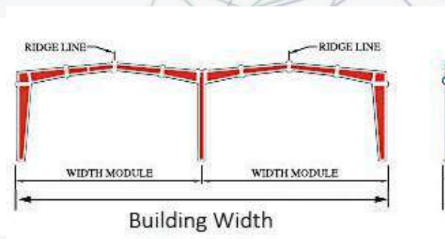
MULTI-GABLE
