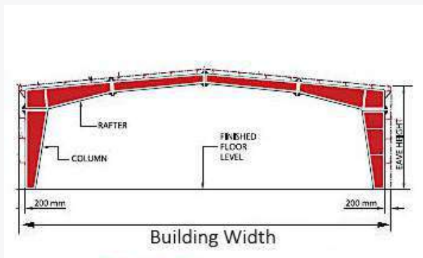
SINGLE SPAN
