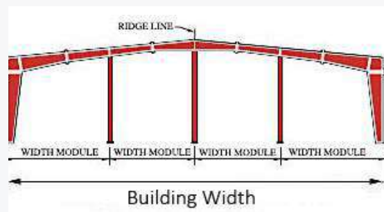
MULTI-SPAN '3'
