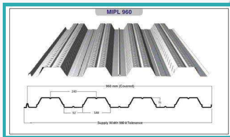
DECKING PROFILE
